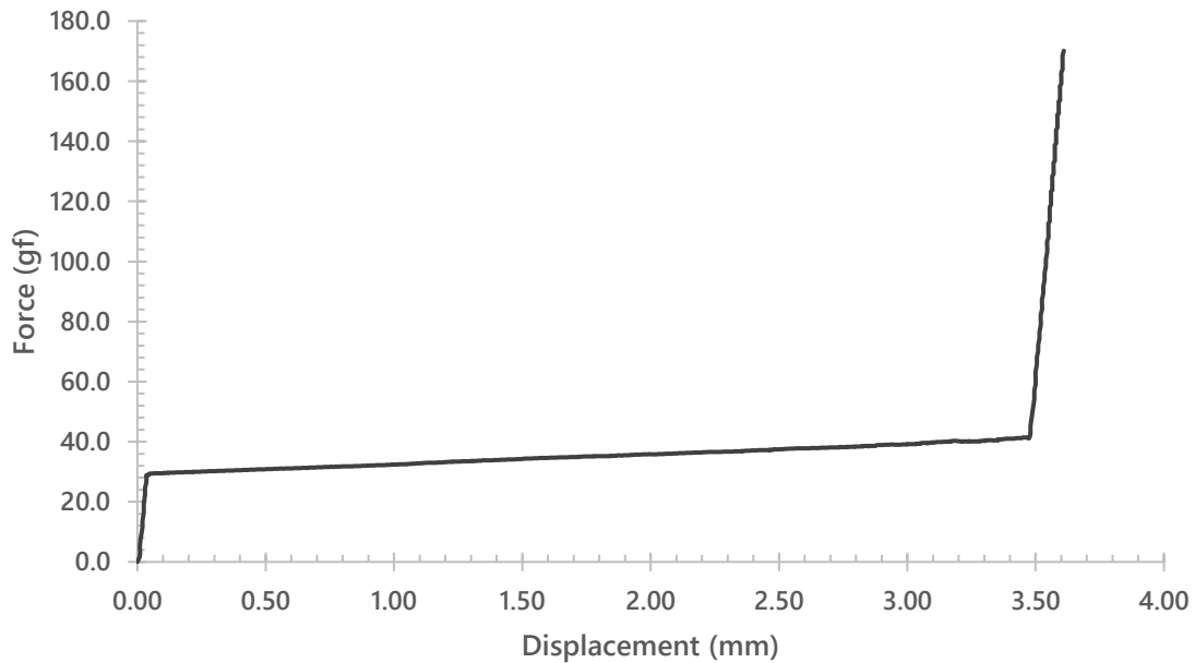
Gateron Milky Yellow HE (Upstroke)
